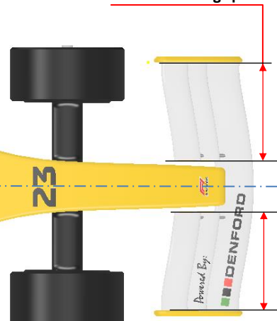
T8.5.1 Front wing span
